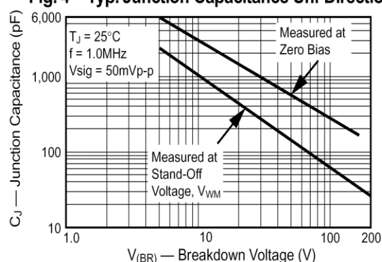
Fig. 4 – Typ. Junction Capacitance Uni-Directional
