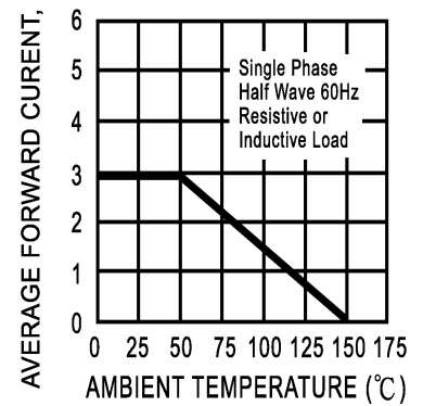
FIG. 2 - TYPICAL FORWARD CURRENT DERATING CURVE
