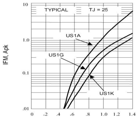
Fig. 2-FORWARD CHARACTERISTICS
