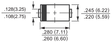
SMC (DO-214AB)
